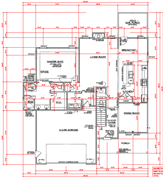
FIRST FLOOR PLAN SCALE 1/8" = 1'-0"
